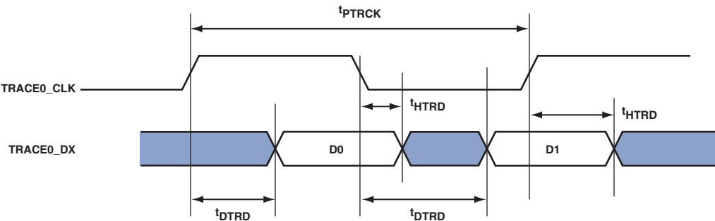
Figure 64. Trace Timing
