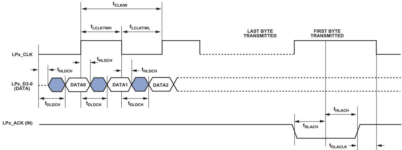
Figure 15. LPs DDR—Transmit
