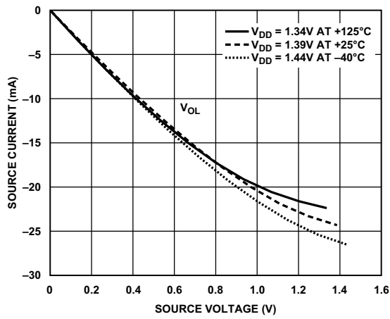
Figure 70. Driver Type B and Driver Type C (DDR3L Drive Strength 40 \Omega )
