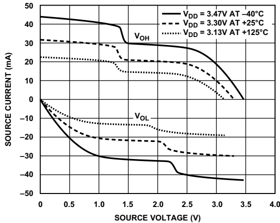
Figure 66. Driver Type A Current for All Pins Operating Above 62.5 MHz and Less Than or Equal to 125 MHz (3.3 V V_{DD\_EXT} )
