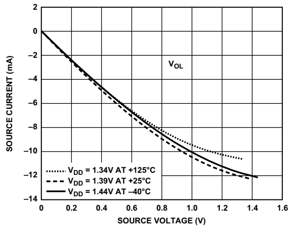
Figure 80. Driver Type B and Driver Type C (DDR3L Drive Strength 90 \Omega )
