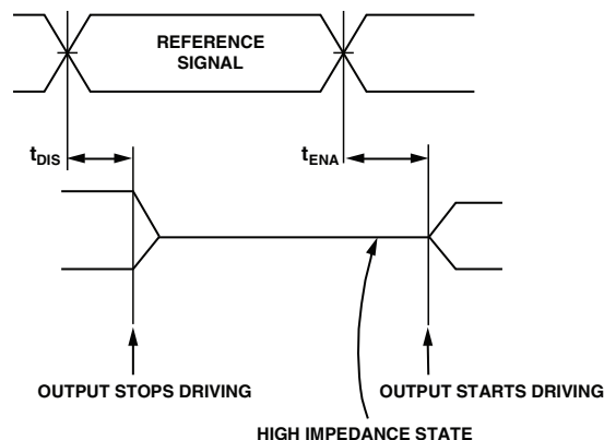
Figure 84. Output Enable/Disable
