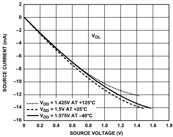
Figure 76. Driver Type B and Driver Type C (DDR3 Drive Strength 90 \Omega )
