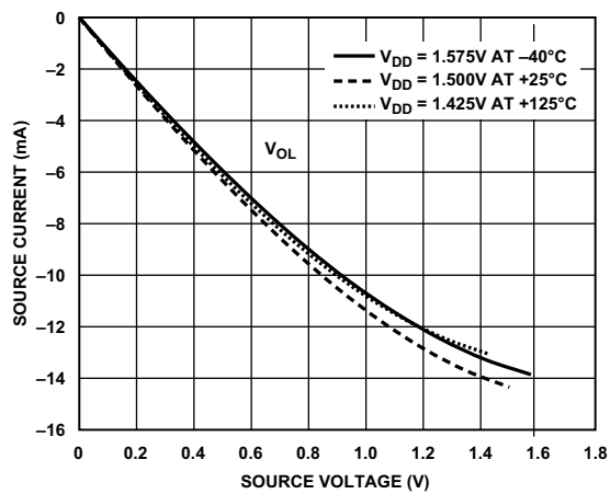
Figure 78. Driver Type B and Driver Type C (DDR3 Drive Strength 100 \Omega )
