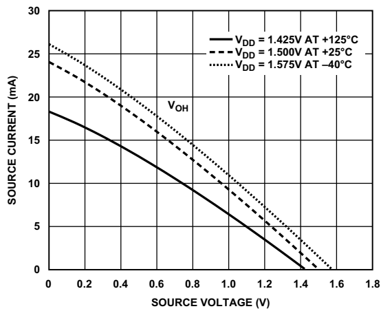
Figure 71. Driver Type B and Driver Type C (DDR3 Drive Strength 60 \Omega )
