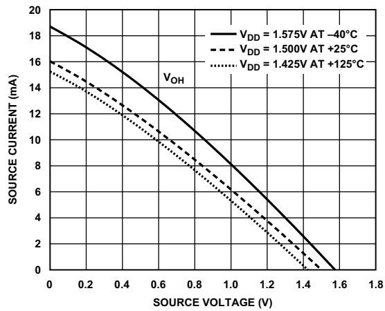
Figure 77. Driver Type B and Driver Type C (DDR3 Drive Strength 100 \Omega )
