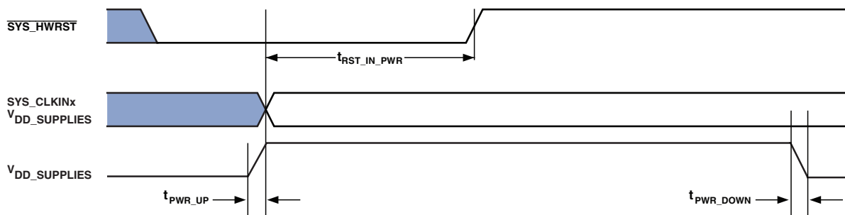
Figure 9. Power-Up Reset Timing
