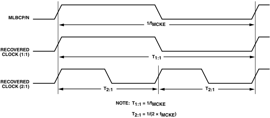
Figure 58. MLB 6-Pin Clock Definitions
