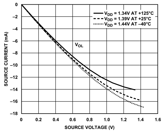
Figure 74. Driver Type B and Driver Type C (DDR3L Drive Strength 60 \Omega )
