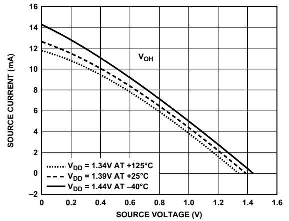
Figure 79. Driver Type B and Driver Type C (DDR3L Drive Strength 90 \Omega )
