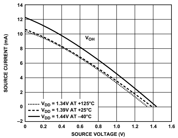
Figure 81. Driver Type B and Driver Type C (DDR3L Drive Strength 100 \Omega )
