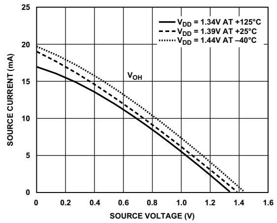
Figure 73. Driver Type B and Driver Type C (DDR3L Drive Strength 60 \Omega )
