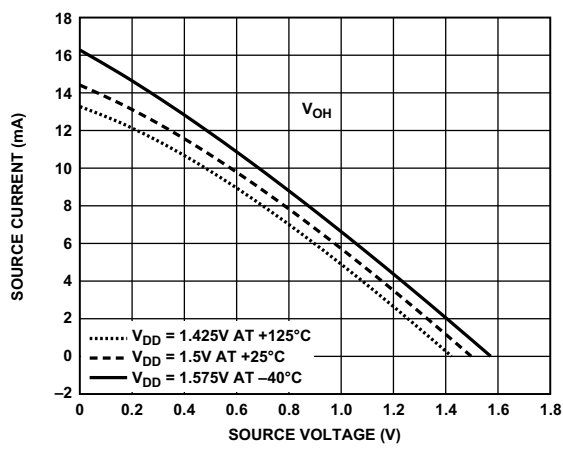
Figure 75. Driver Type B and Driver Type C (DDR3 Drive Strength 90 \Omega )
