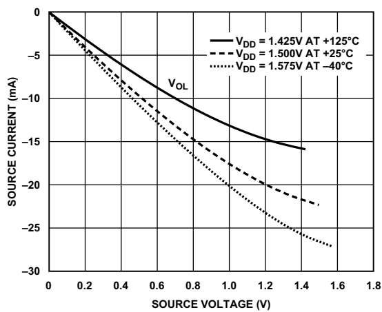
Figure 72. Driver Type B and Driver Type C (DDR3 Drive Strength 60 \Omega )
