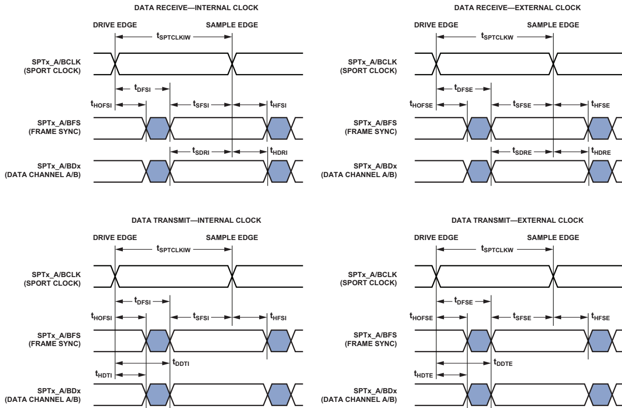
Figure 16. SPORTs
