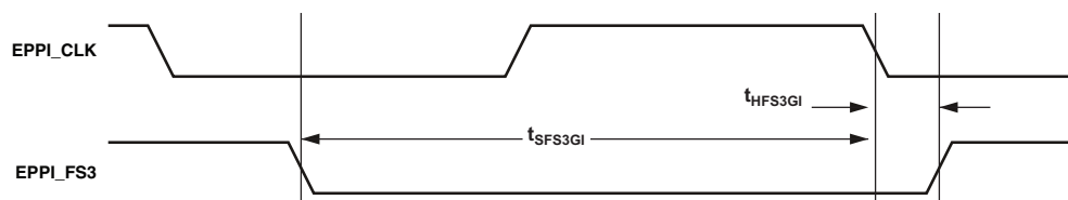
Figure 46. Clock Gating Mode with Internal Clock and External Frame Sync Timing
